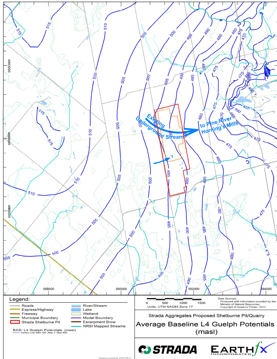
Figure 3.4: Average Baseline Guelph Formation Water Levels
