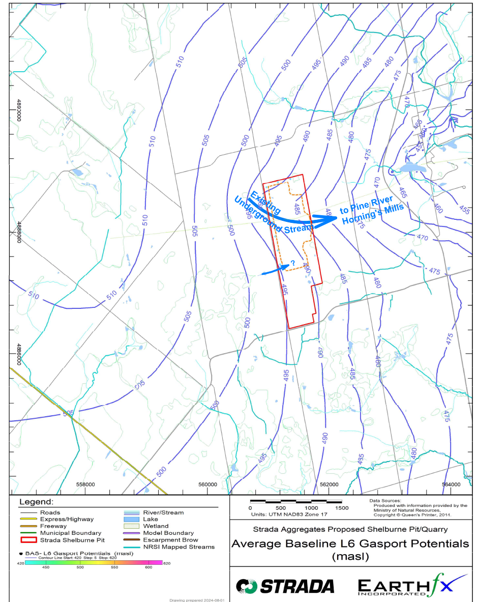
Figure 3.5: Average Gasport Formation Water Levels
